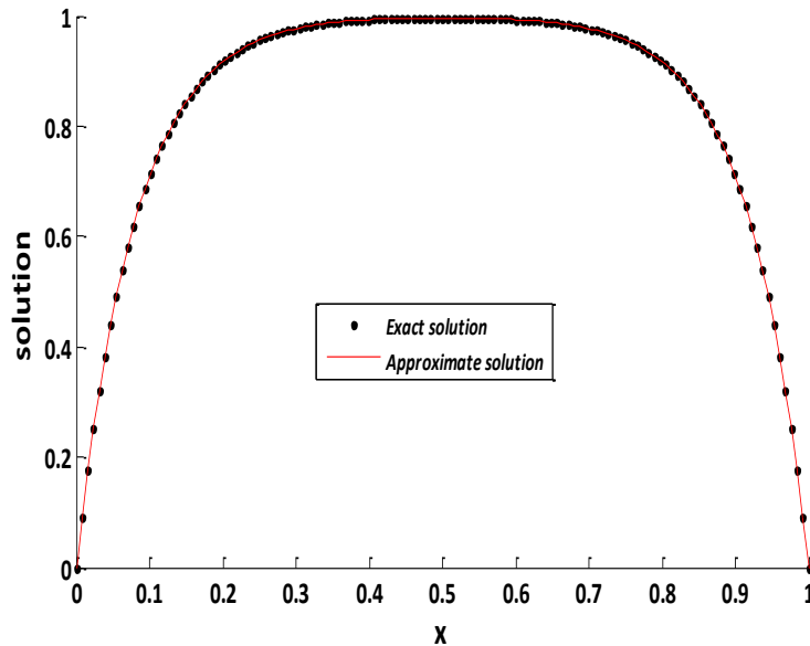
Fig. 4: Comparison of solutions for Problem 2, Method 3.2, \varepsilon = \frac{1}{128} , h = \frac{1}{128}
