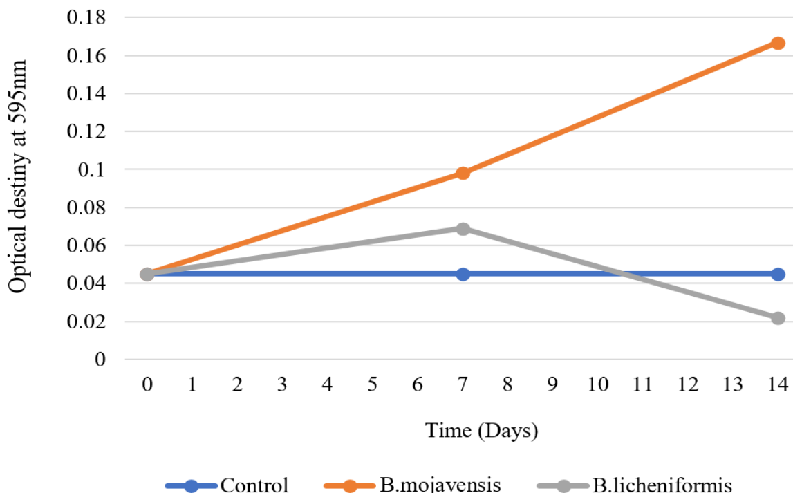
Figure 5. Growth of B. mojavensis and B. licheniformis in BHMS medium supplemented with nitrogen mineral according to (O.D value) at 595 nm (Gasoline concentration 0.01ml/10ml) for 14 days of incubation against BHMS medium as control.
