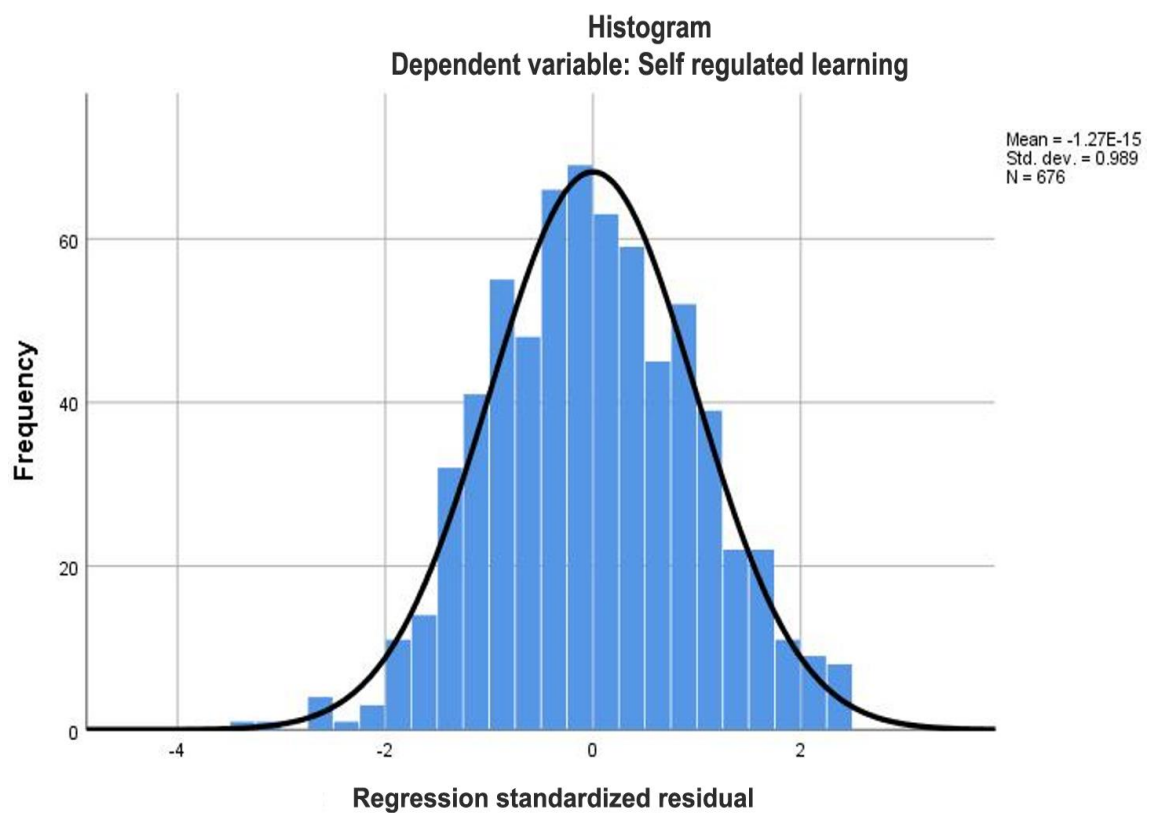
Figure 1. Histogram regression standardized residual.
