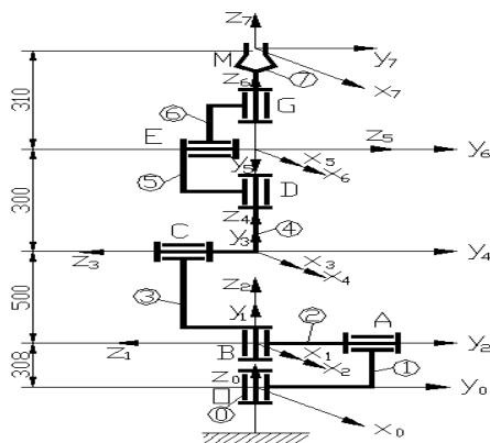
Fig-1. KS of a medical robot with designated Denavit-Hartenberg coordinate systems
