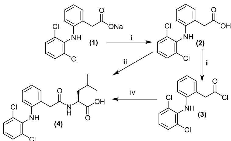
Scheme 1: reagent and conditions; i- H 2 O/ dil-HCl., ii-SOCl 2 , iii-L-Leu/fusion, iv-L-Leu/THF/TEA.
