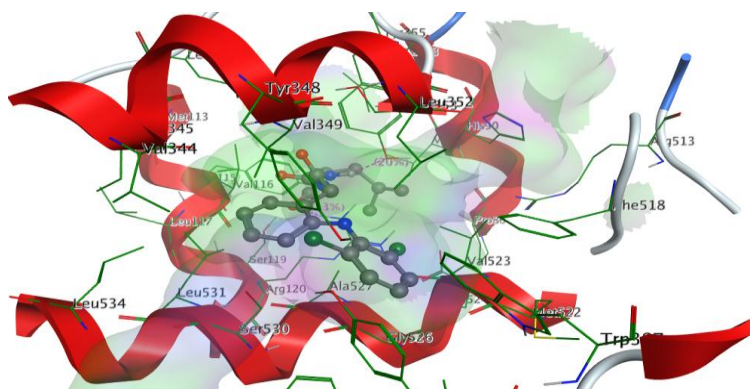
Fig-2. The compound (4) Docked into the active site of COX-2. using MOE tool.
