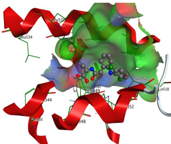
Fig-2. The compound (1) Docked into the active site of COX-2. using MOE tool.
