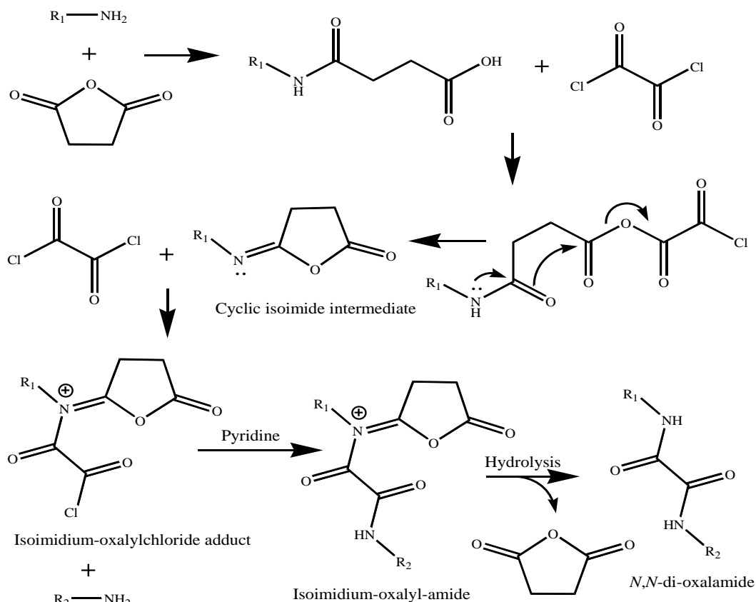
Scheme-1. Proposed mechanism of N,N -di-oxalamide synthesis Habash and Taha [12].
