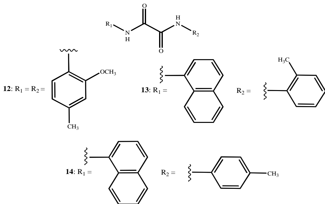
Fig-2. Previously synthesized N,N -di-oxalamide derivatives 7-9 Habash and Taha [12].
