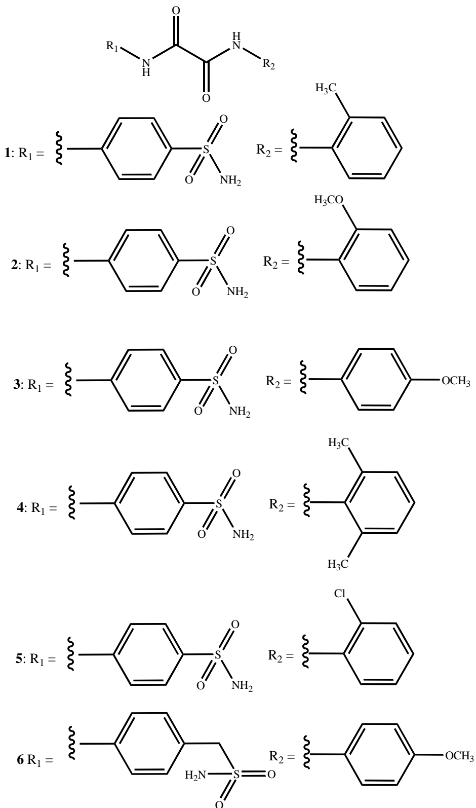
Fig-1. Structures of N,N -di-oxalamide derivatives 1-6 (Under Experimental Section 2.2).
