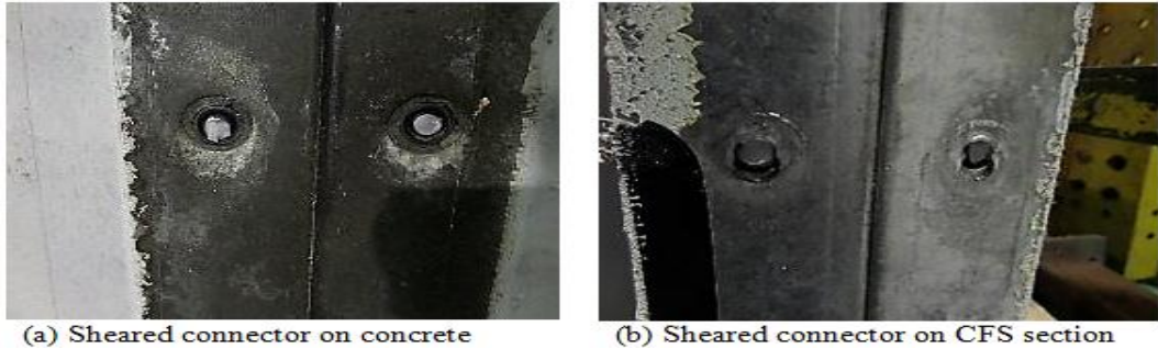
Figure-8. Failure mode of specimens with M12 bolt
