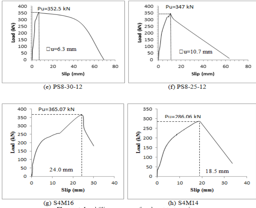
Figure-3. Load-Slip responses of push-out test specimens
