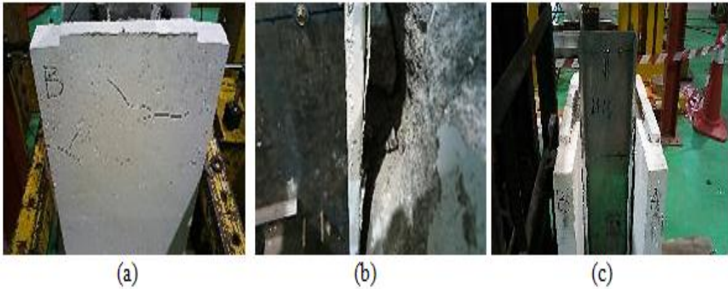
Figure-5. Failure modes of S4M16 specimen [(a) Minor cracks, (b) Concrete crushing, (c) Intact CFS section]
