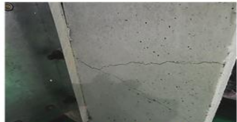
(b) Cracks underneath slab
