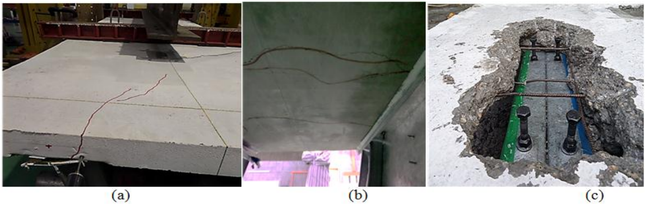
Figure-8. Failure modes of composite beam specimens: [(a) Concrete cracks on slab surface, (b) Transverse cracks beneath the slab, (c) Non-deformed shear connector]
