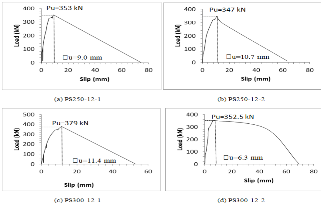
Figure-5. Load-slip responses of push-out specimens
