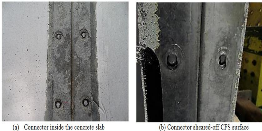
Figure-6. Failure mode of specimens with M12 bolted shear connector
