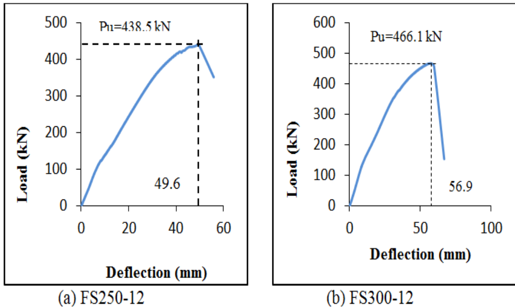
Figure-7. Load-mid-span deflection of composite beam specimens
