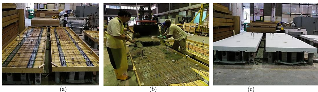
Figure-2. Preparation of full-scale test specimens [(a) samples formwork, (b) samples casting, (c) finished samples]
