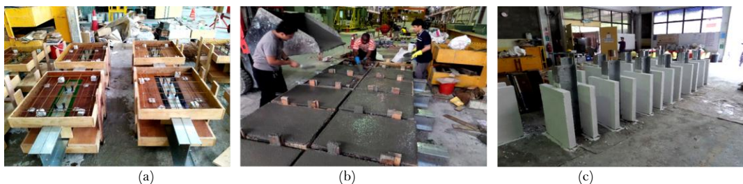
Figure-1. Preparation of push-out test specimens [(a) samples formwork, (b) samples casting, (c) finished samples]
