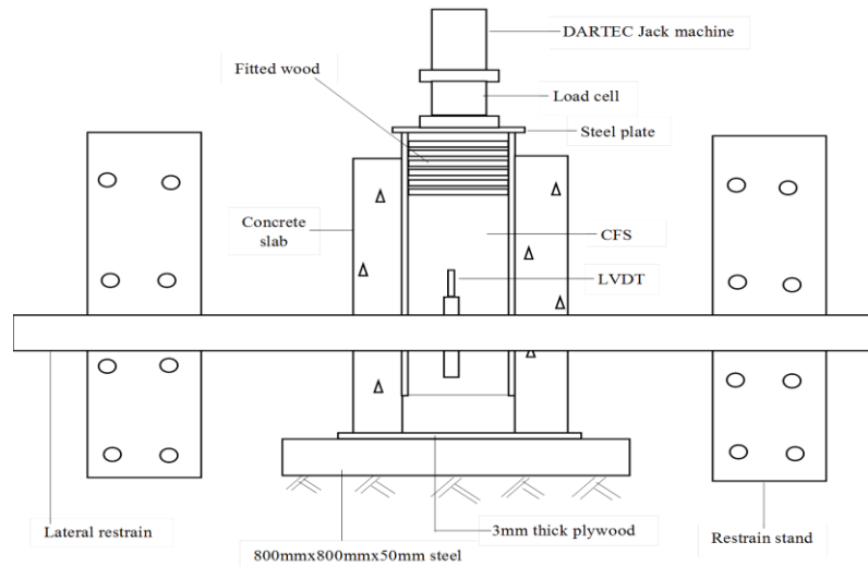
Figure-3. Push-out test set up
