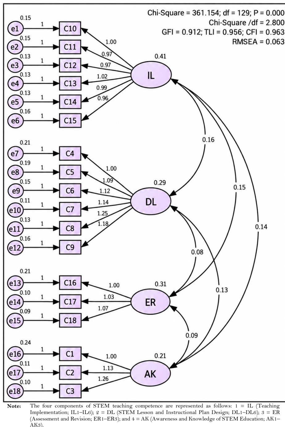
Figure 1. The CFA results.
